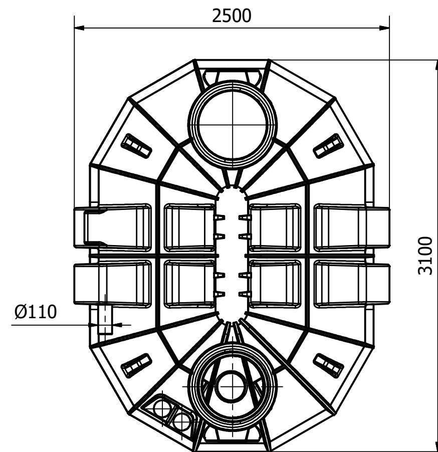
Top View
