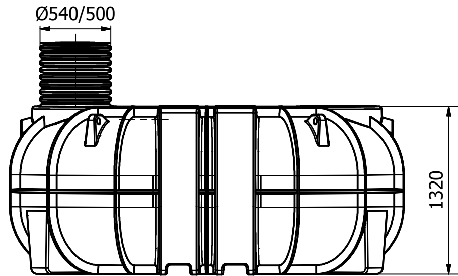
Right View
